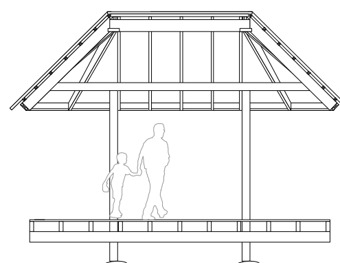
structural principle: stone - column - floor - roof
