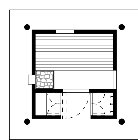
floorplan (12m2)
