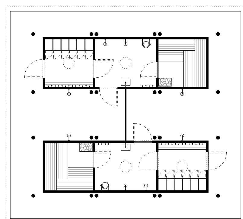
floorplan (90m2)
